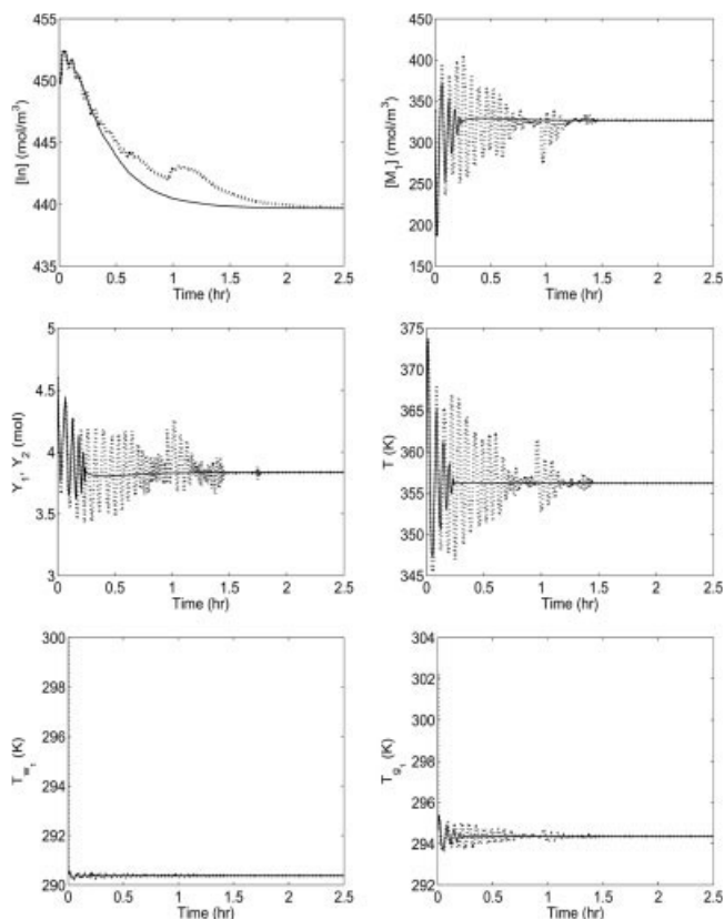
Figure 9. Evolution of the closed-loop state profiles under primary control configuration under continuous measurements (solid lines), and sensor data loss rate of 0.75 (dotted lines).
